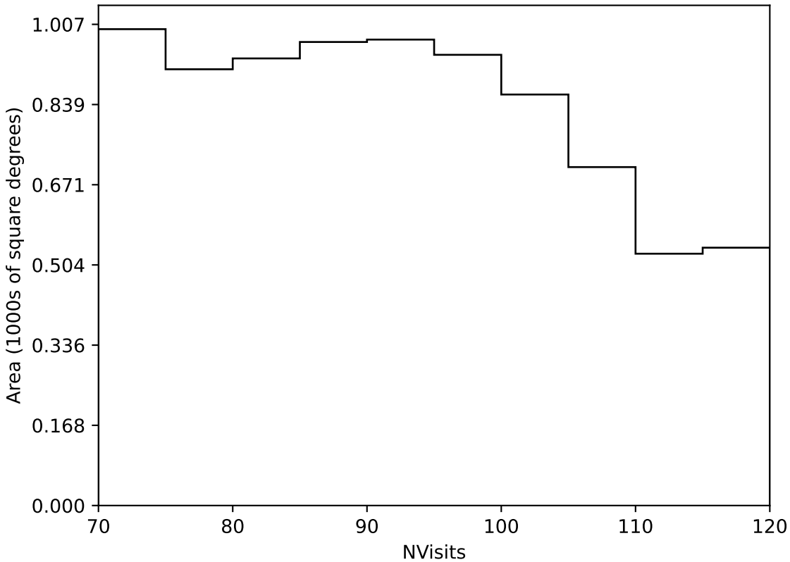
roll_pause_mjdp60_v3.4_10yrs Yr 3-4 all bands: NVisits
