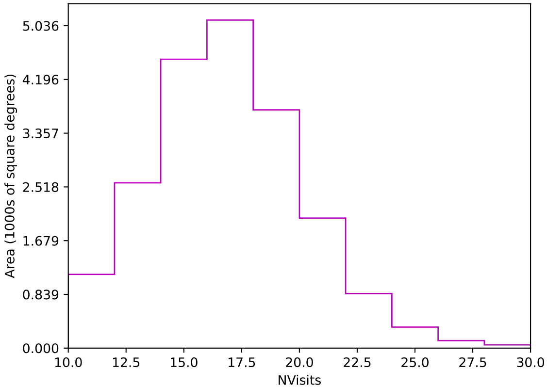
roll_pause_mjdp60_v3.4_10yrs Yr 1 z band: NVisits
