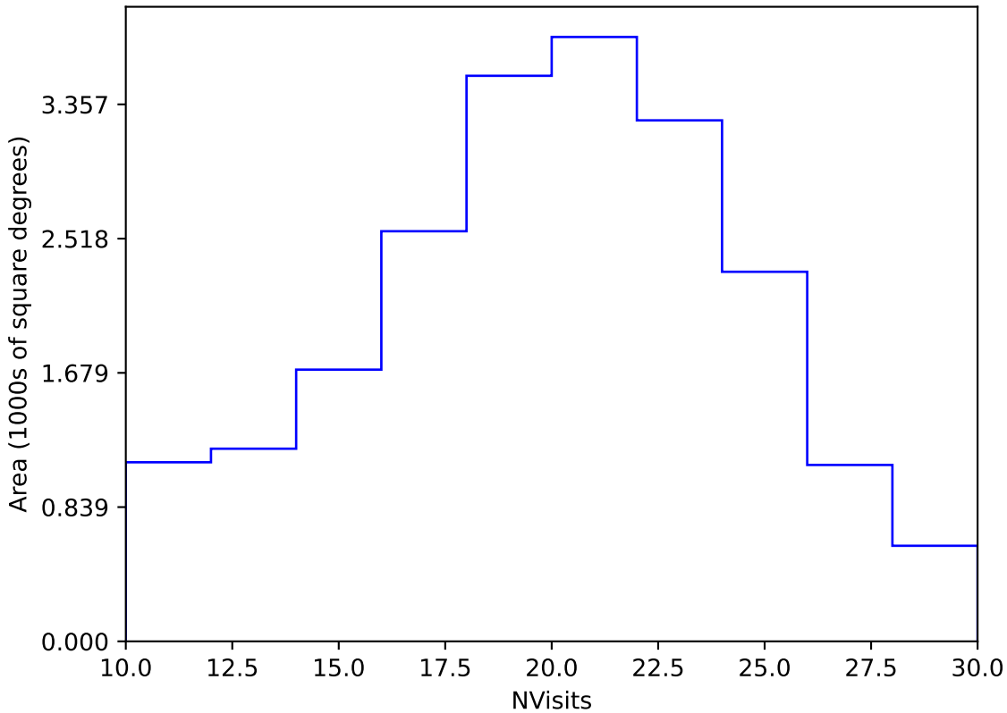
roll_pause_mjdp60_v3.4_10yrs Yr 1 y band: NVisits
