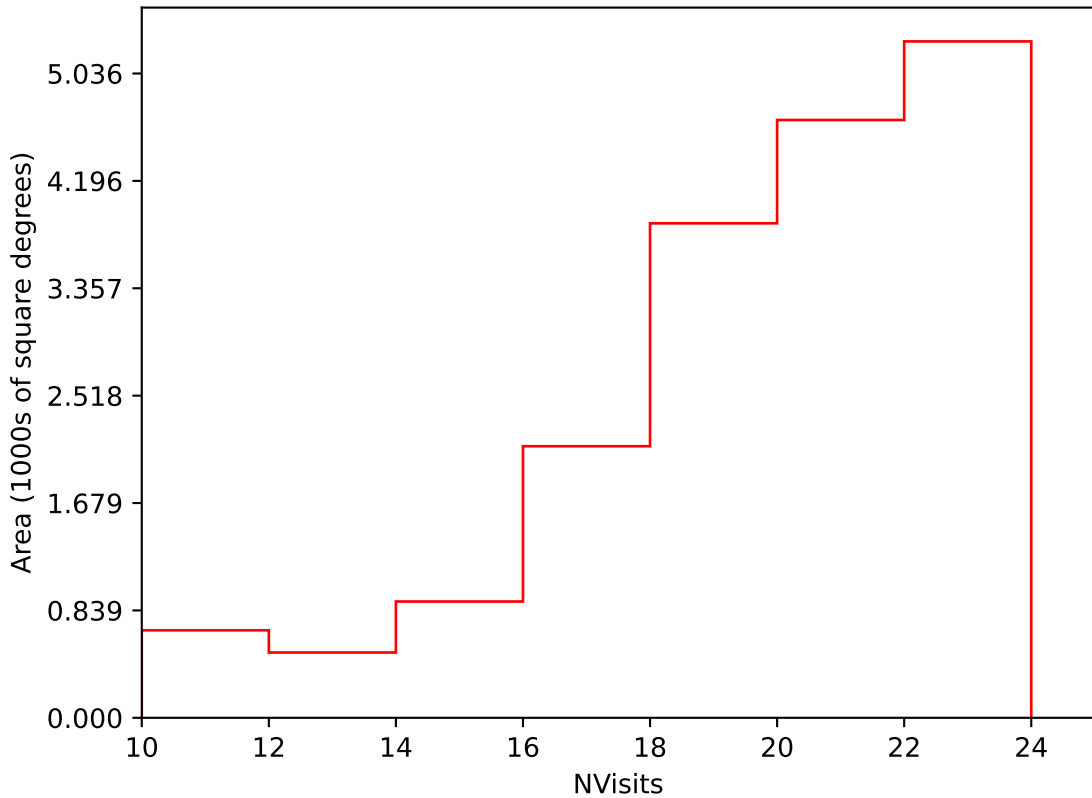
roll_pause_mjdp60_v3.4_10yrs Yr 1 i band: NVisits
