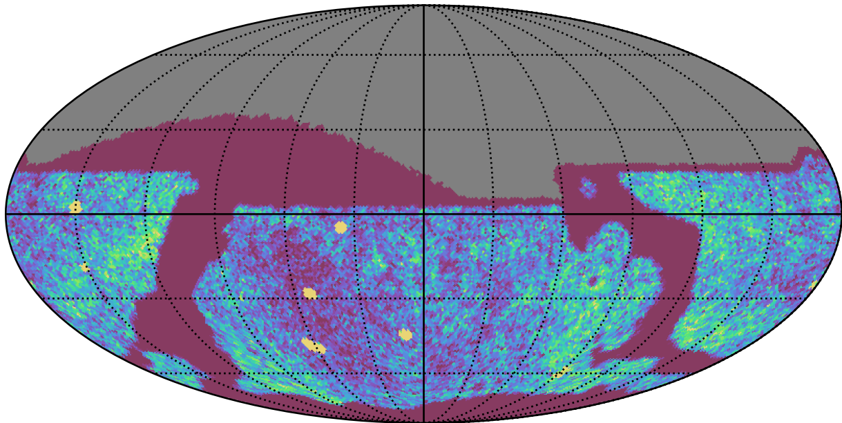
roll_pause_mjdp60_v3.4_10yrs Yr 1 all bands: NVisits
