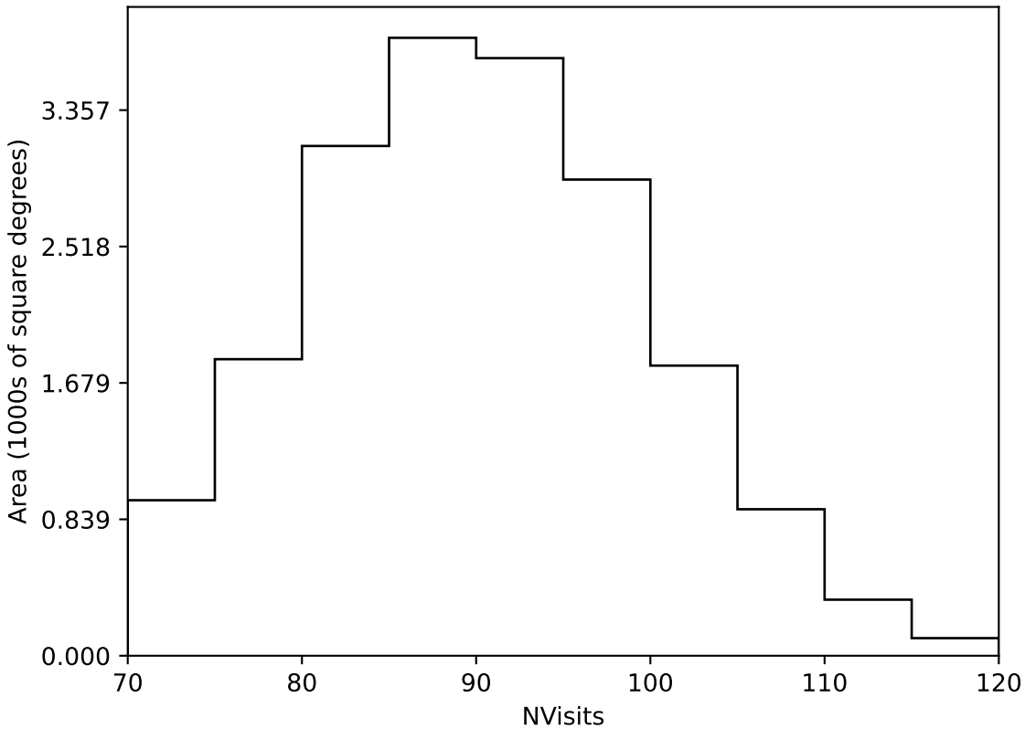
roll_pause_mjdp60_v3.4_10yrs Yr 1 all bands: NVisits
