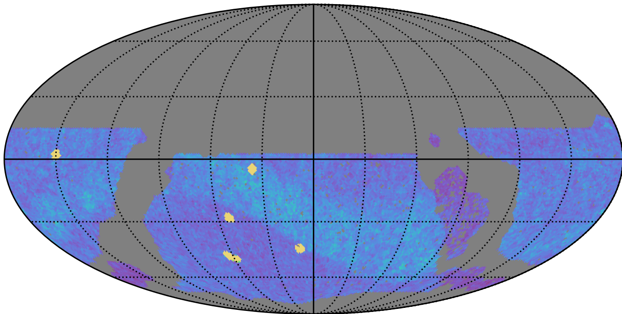
roll_pause_mjdp60_v3.4_10yrs WFD z band: NVisits
