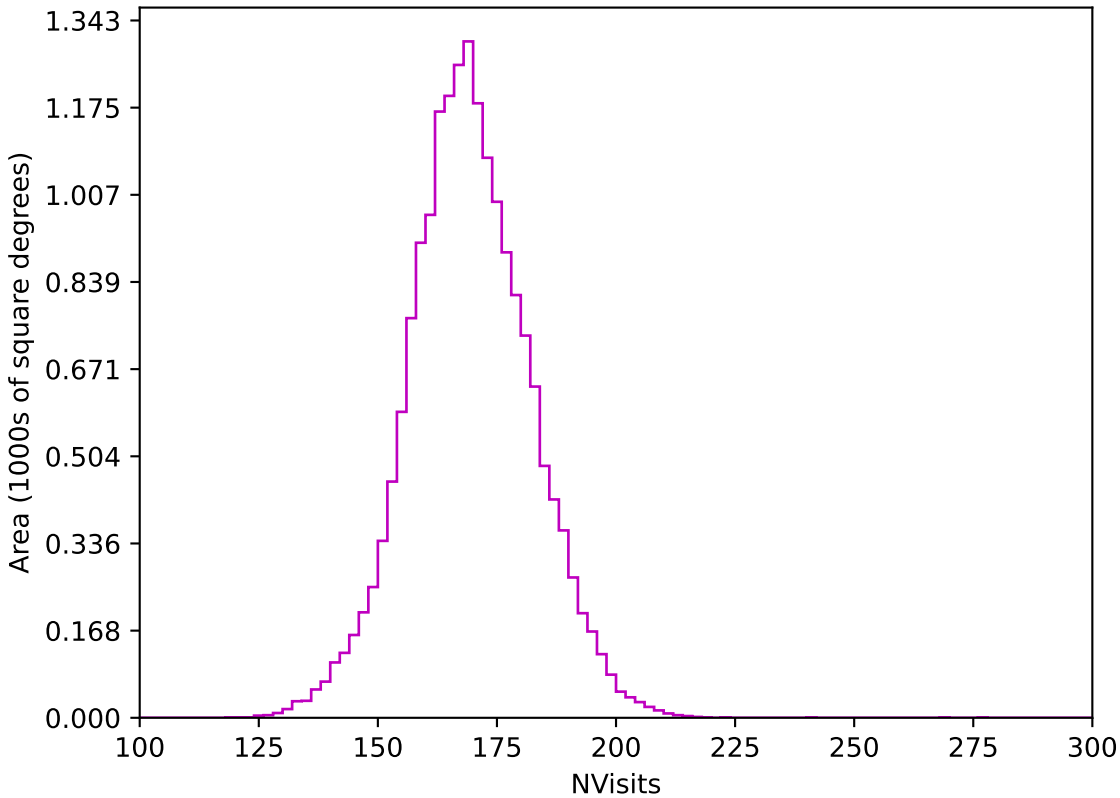
roll_pause_mjdp60_v3.4_10yrs WFD z band: NVisits
