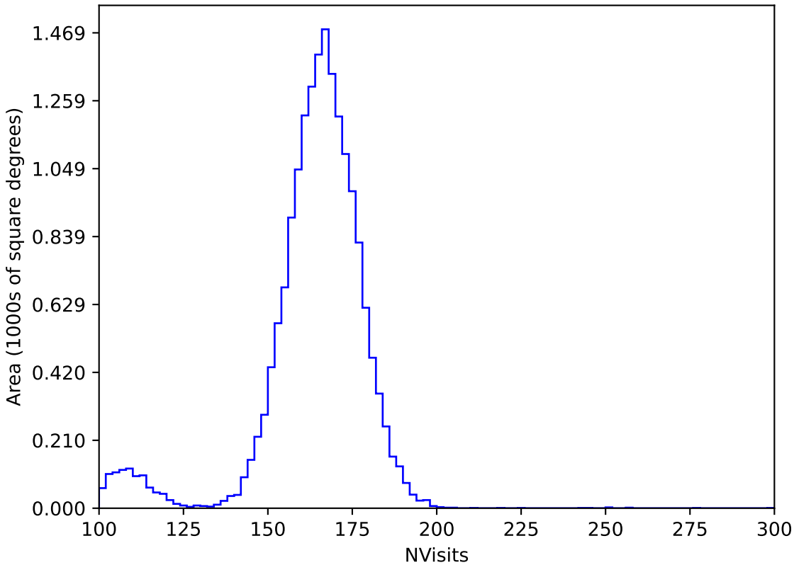
roll_pause_mjdp60_v3.4_10yrs WFD y band: NVisits
