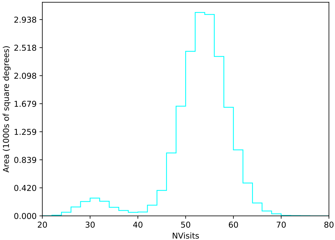
roll_pause_mjdp60_v3.4_10yrs WFD u band: NVisits
