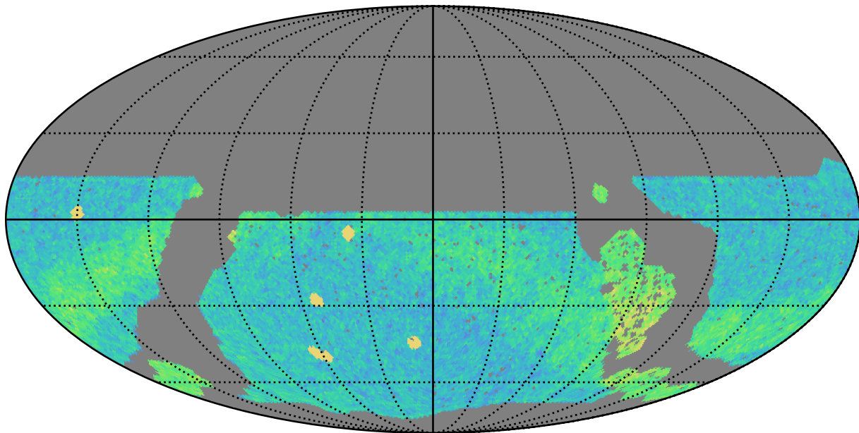
roll_pause_mjdp60_v3.4_10yrs WFD r band: NVisits
