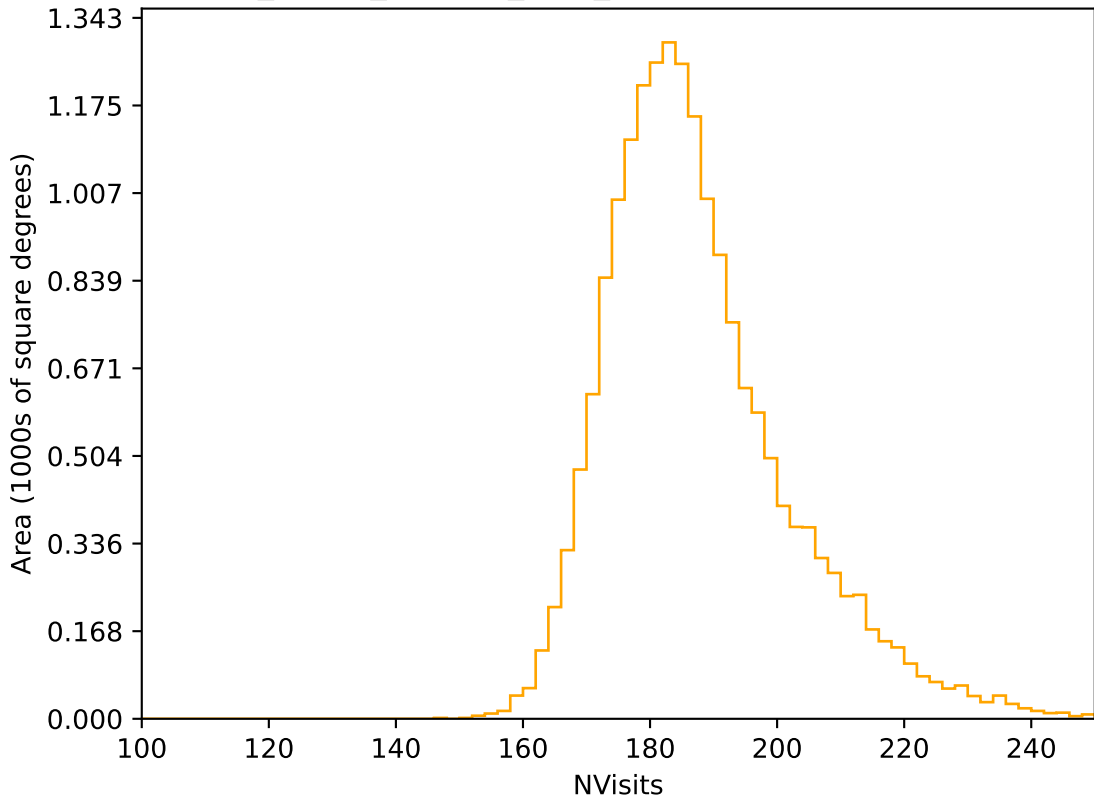
roll_pause_mjdp60_v3.4_10yrs WFD r band: NVisits
