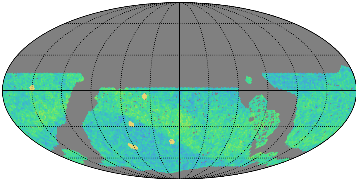
roll_pause_mjdp60_v3.4_10yrs WFD i band: NVisits
