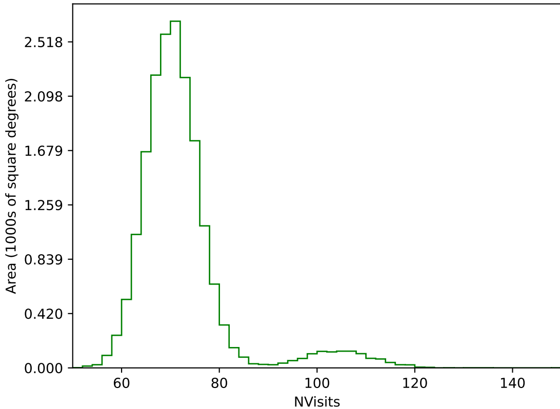
roll_pause_mjdp60_v3.4_10yrs WFD g band: NVisits
