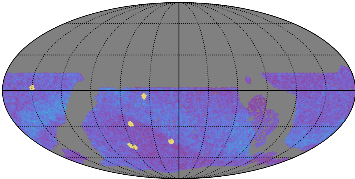
roll_pause_mjdp60_v3.4_10yrs WFD all bands: NVisits
