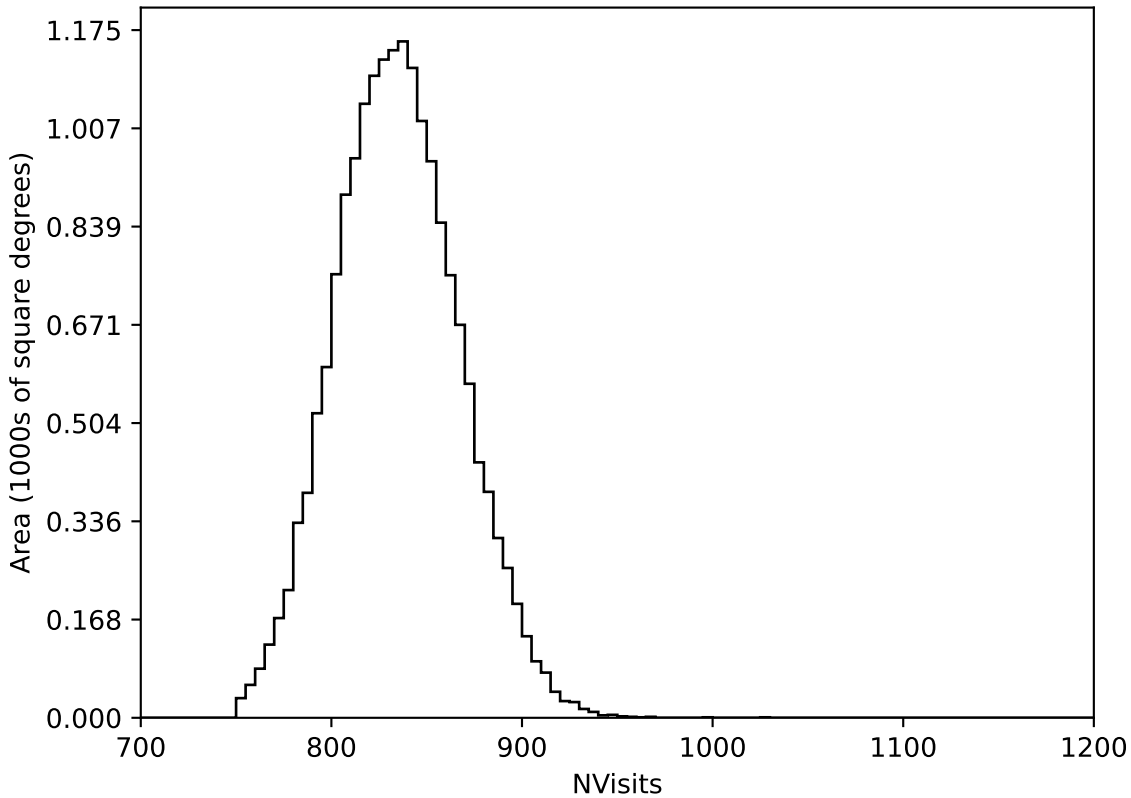
roll_pause_mjdp60_v3.4_10yrs WFD all bands: NVisits
