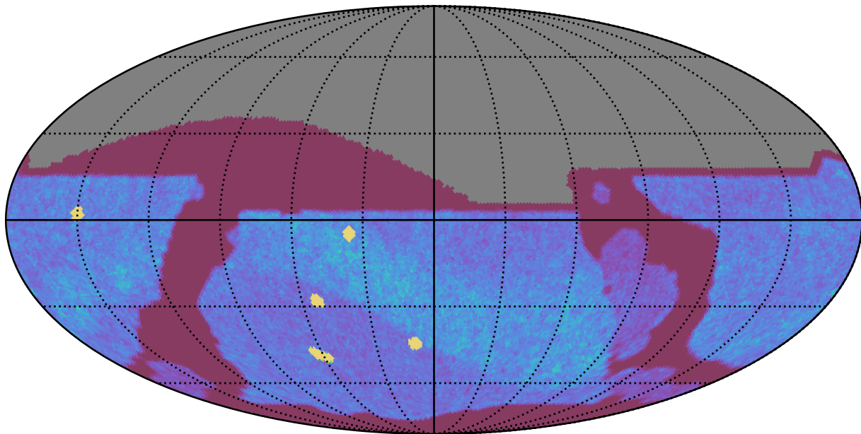
roll_pause_mjdp60_v3.4_10yrs All sky z band: NVisits
