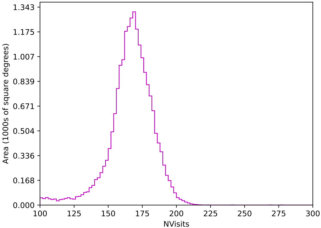
roll_pause_mjdp60_v3.4_10yrs All sky z band: NVisits
