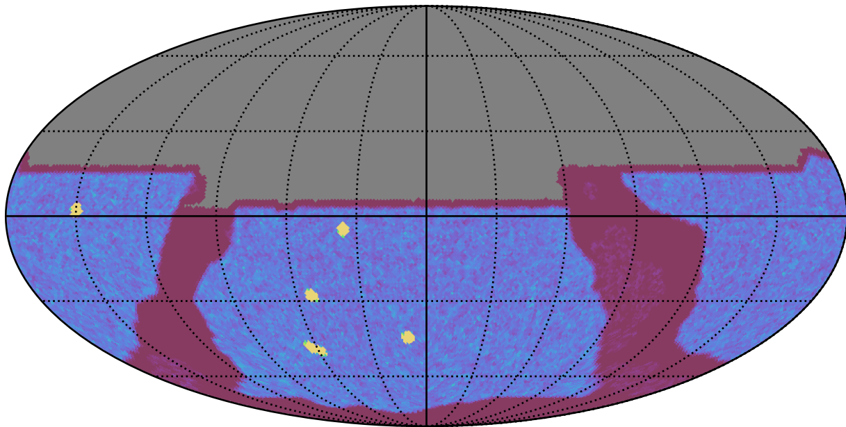
roll_pause_mjdp60_v3.4_10yrs All sky y band: NVisits
