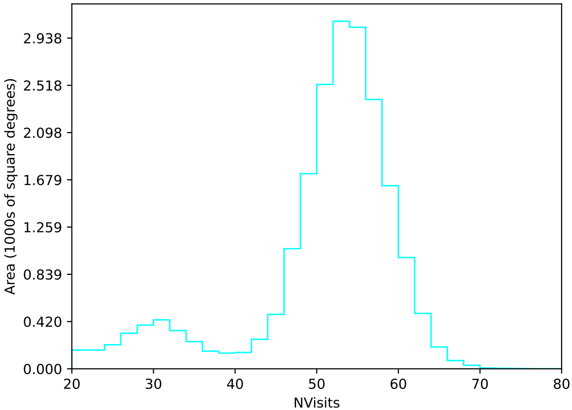
roll_pause_mjdp60_v3.4_10yrs All sky u band: NVisits
