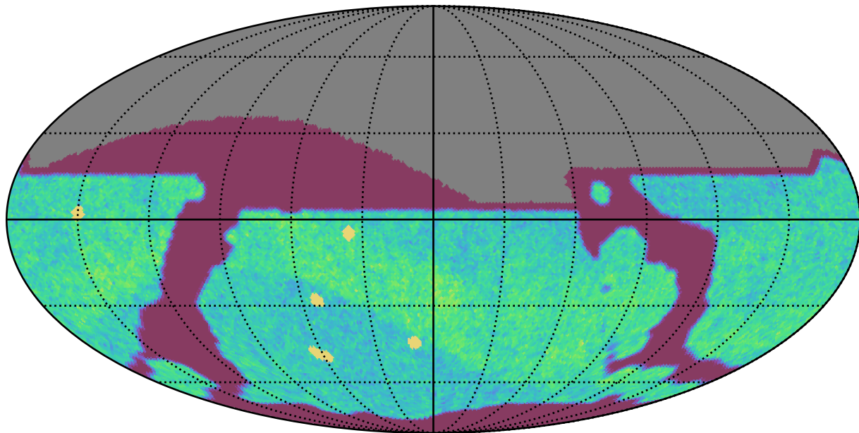
roll_pause_mjdp60_v3.4_10yrs All sky i band: NVisits
