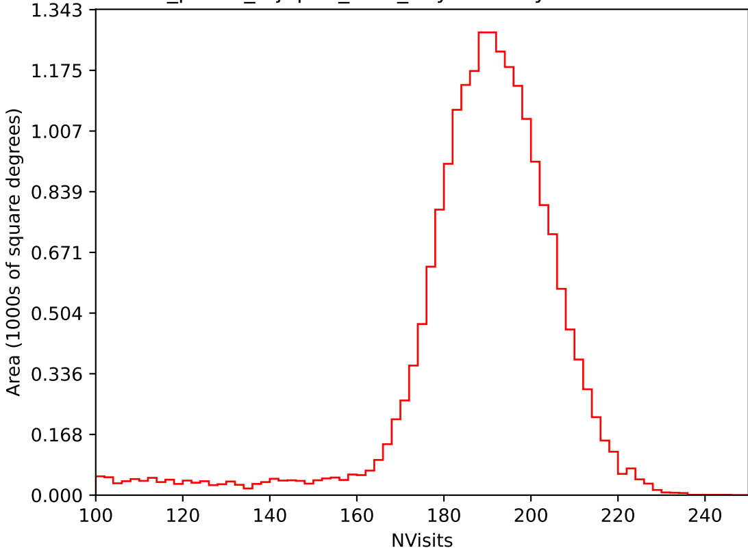
roll_pause_mjdp60_v3.4_10yrs All sky i band: NVisits
