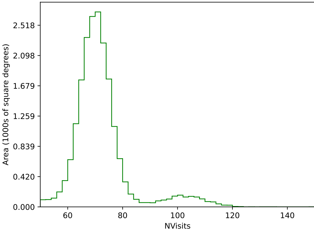
roll_pause_mjdp60_v3.4_10yrs All sky g band: NVisits
