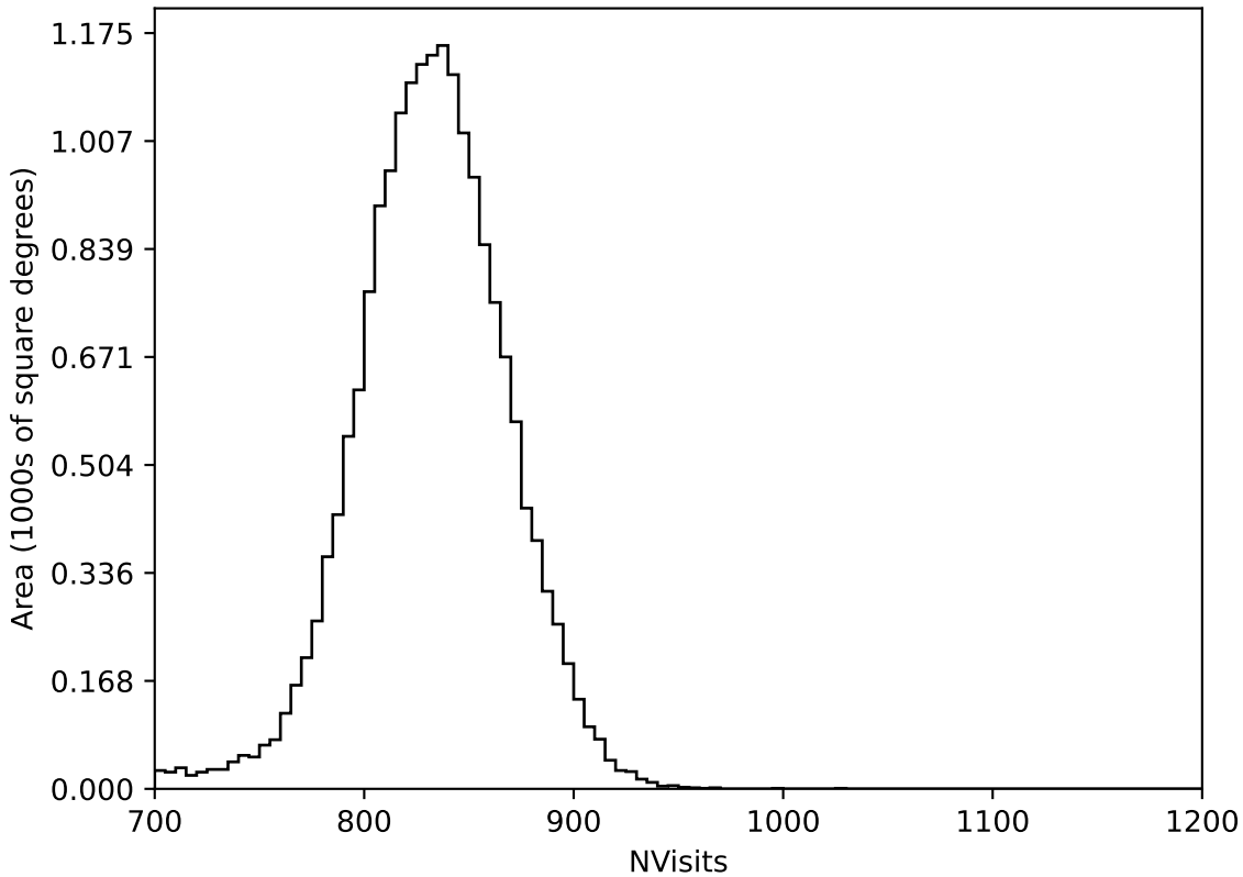
roll_pause_mjdp60_v3.4_10yrs All sky all bands: NVisits
