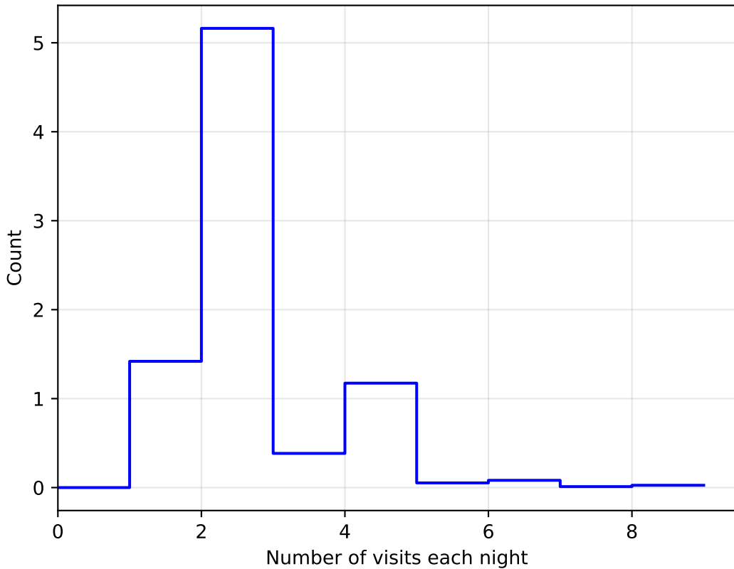
1e6 roll_pause_mjdp60_v3.4_10yrs WFD: NVisitsPerNight
