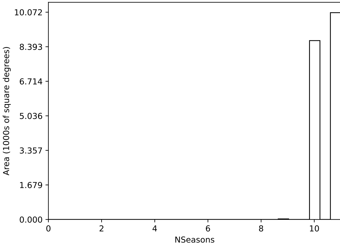
roll_pause_mjdp60_v3.4_10yrs WFD all bands: NSeasons
