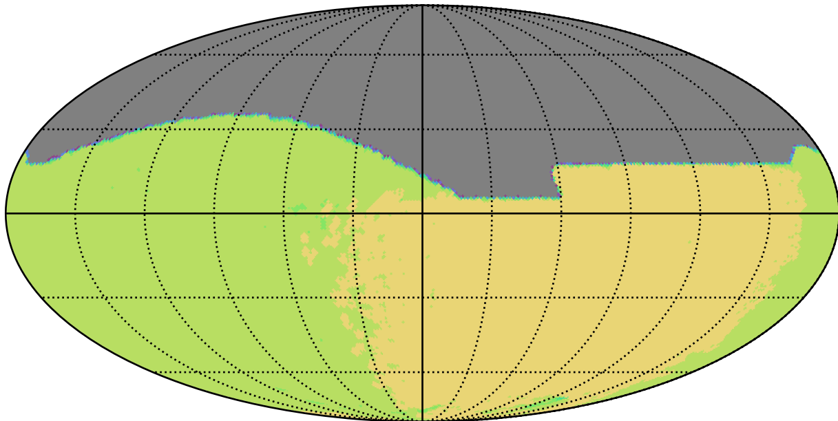
roll_pause_mjdp60_v3.4_10yrs All sky all bands: NSeasons
