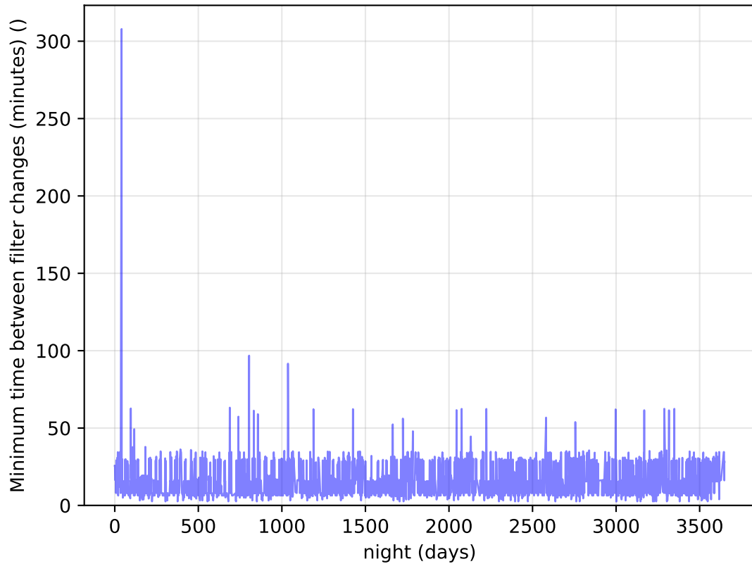
roll_pause_mjdp60_v3.4_10yrs Per Night: Minimum time between filter changes (minutes)
