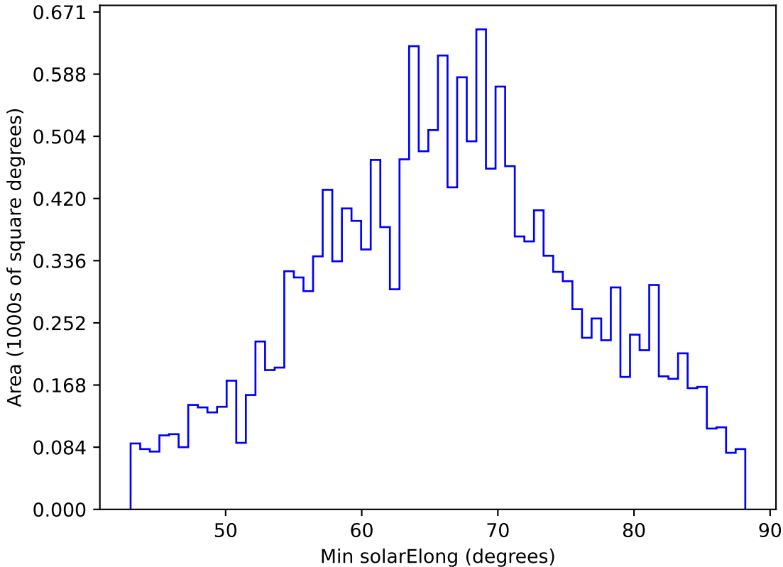
roll_pause_mjdp60_v3.4_10yrs WFD y band: Min solarElong
