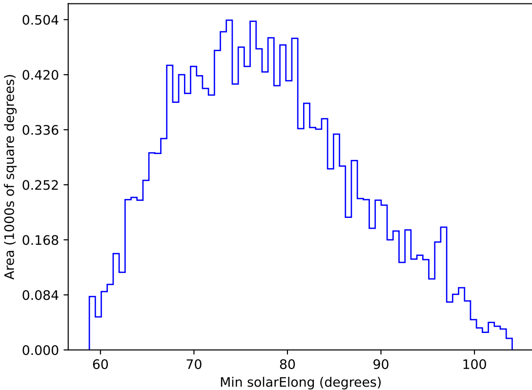
roll_pause_mjdp60_v3.4_10yrs WFD u band: Min solarElong
