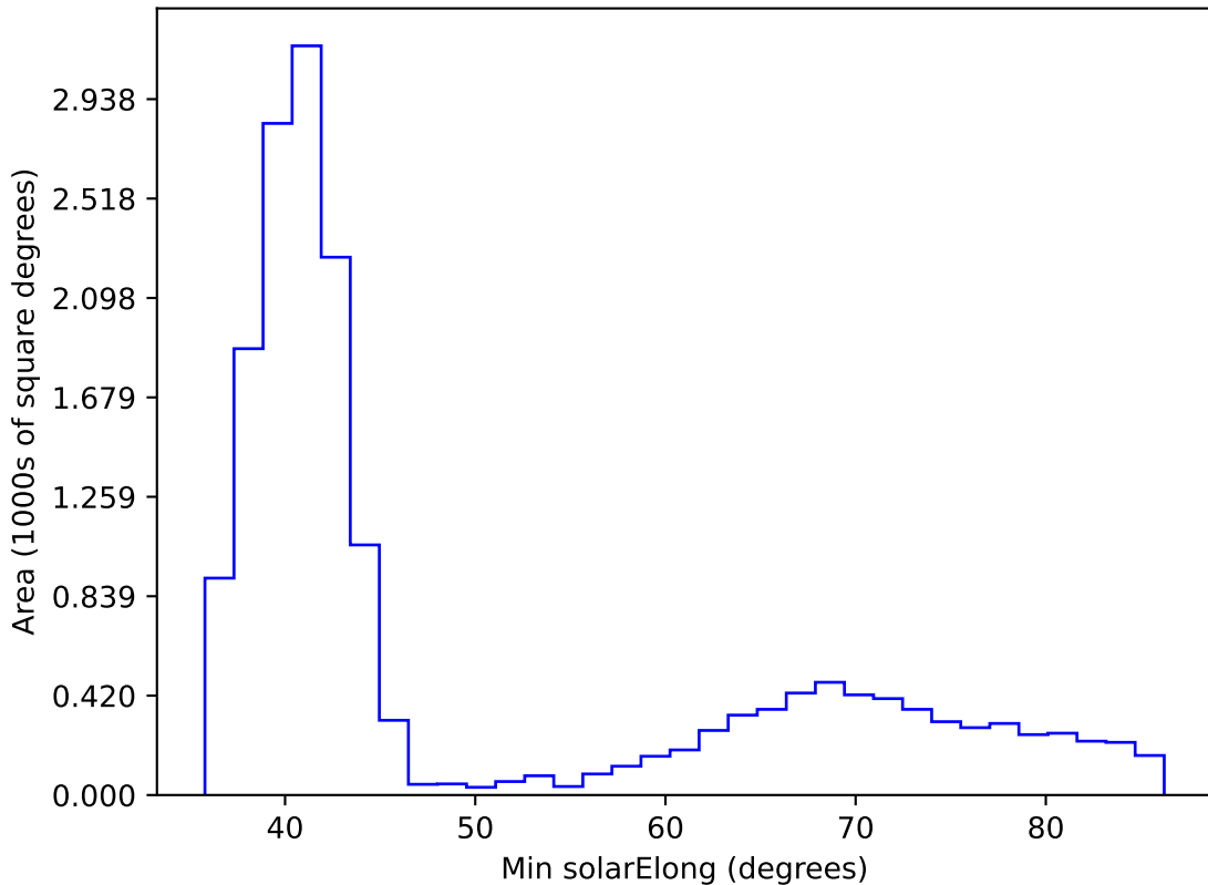
roll_pause_mjdp60_v3.4_10yrs WFD i band: Min solarElong
