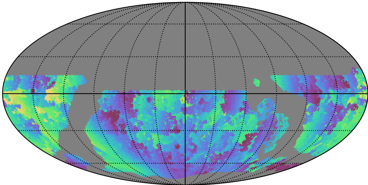
roll_pause_mjdp60_v3.4_10yrs WFD g band: Min solarElong
