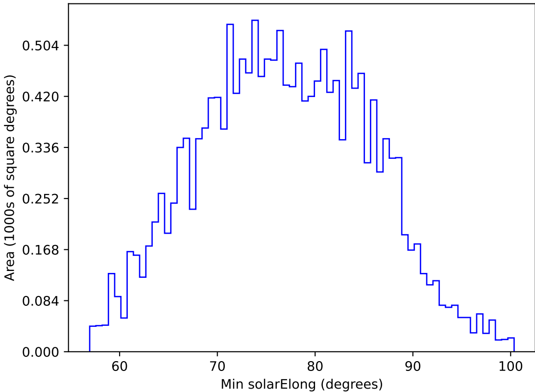
roll_pause_mjdp60_v3.4_10yrs WFD g band: Min solarElong
