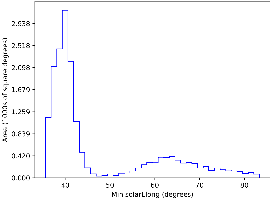
roll_pause_mjdp60_v3.4_10yrs WFD all bands: Min solarElong
