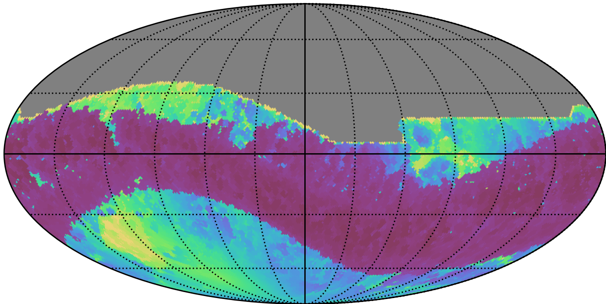
roll_pause_mjdp60_v3.4_10yrs All sky z band: Min solarElong
