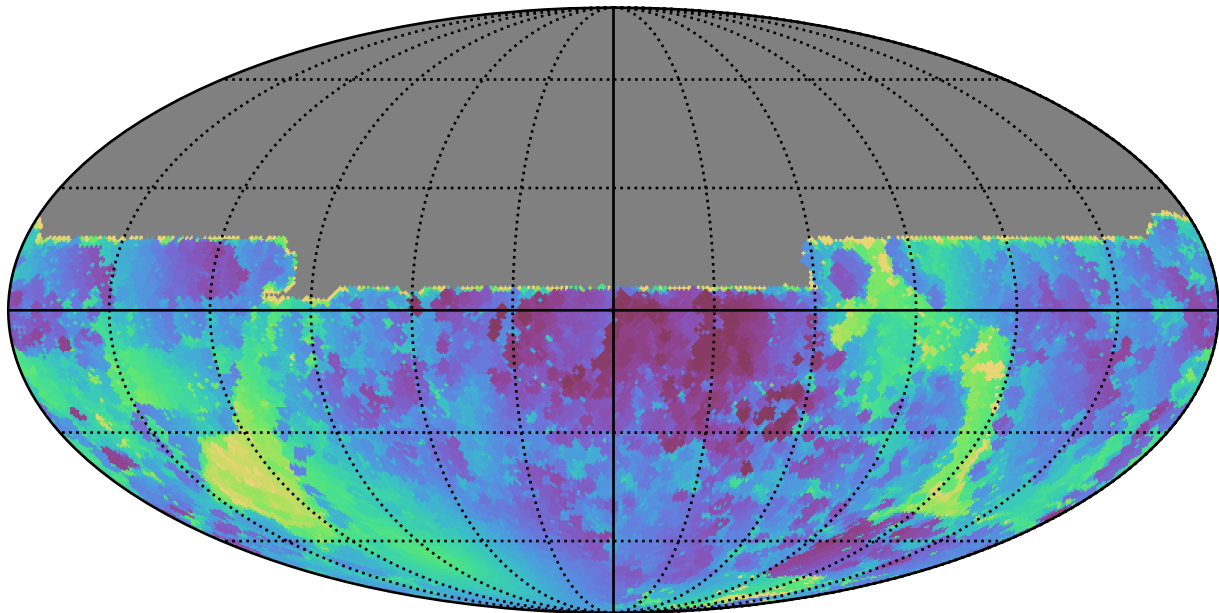
roll_pause_mjdp60_v3.4_10yrs All sky y band: Min solarElong
