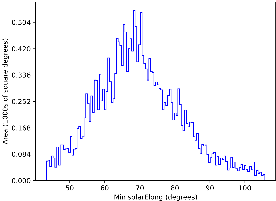
roll_pause_mjdp60_v3.4_10yrs All sky y band: Min solarElong
