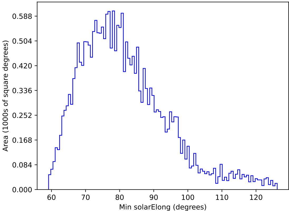
roll_pause_mjdp60_v3.4_10yrs All sky u band: Min solarElong
