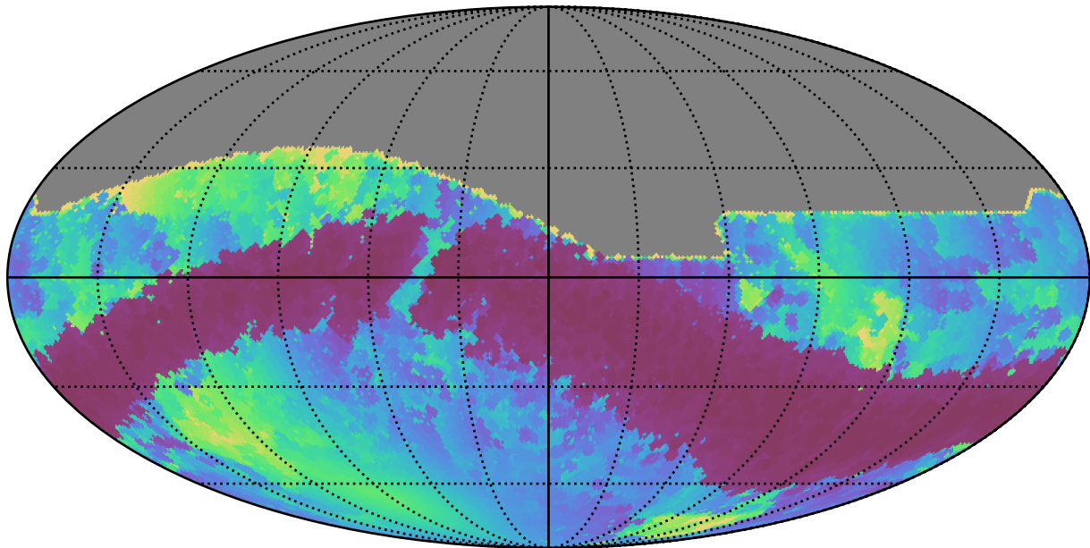
roll_pause_mjdp60_v3.4_10yrs All sky r band: Min solarElong
