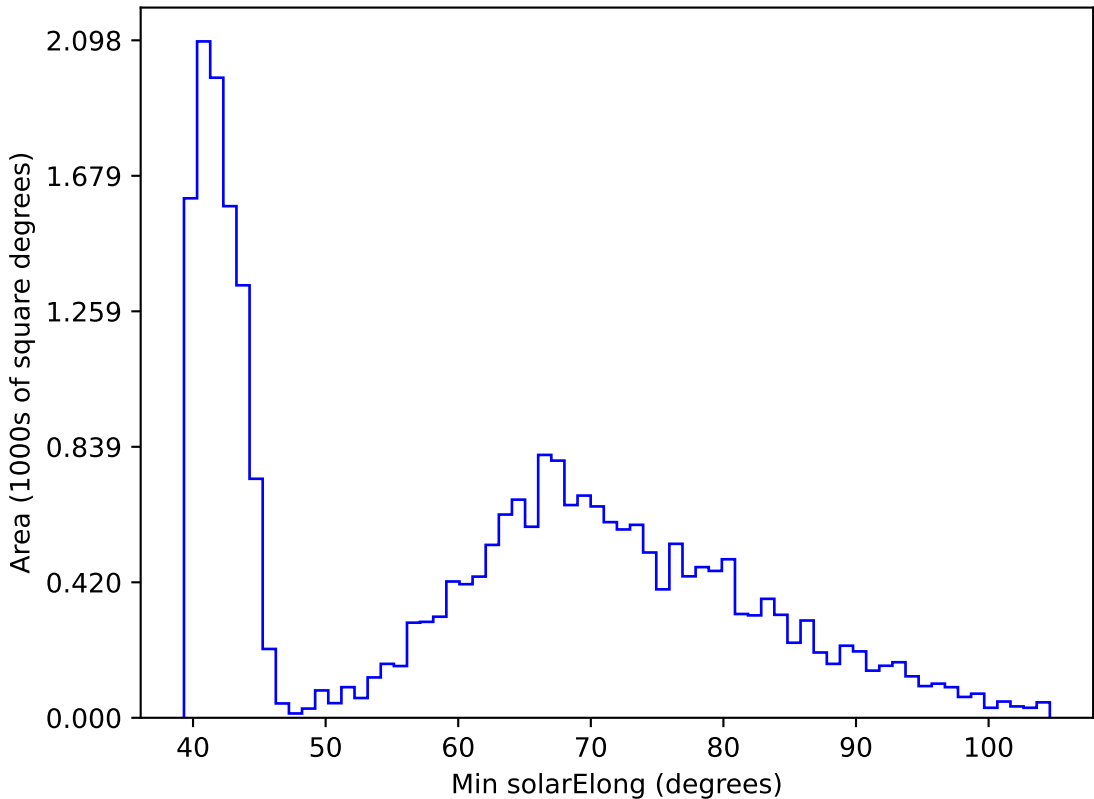
roll_pause_mjdp60_v3.4_10yrs All sky r band: Min solarElong
