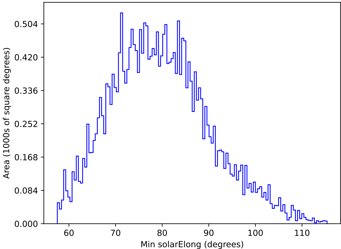
roll_pause_mjdp60_v3.4_10yrs All sky g band: Min solarElong
