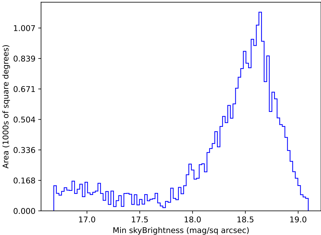
roll_pause_mjdp60_v3.4_10yrs Yr 1 z band: Min skyBrightness
