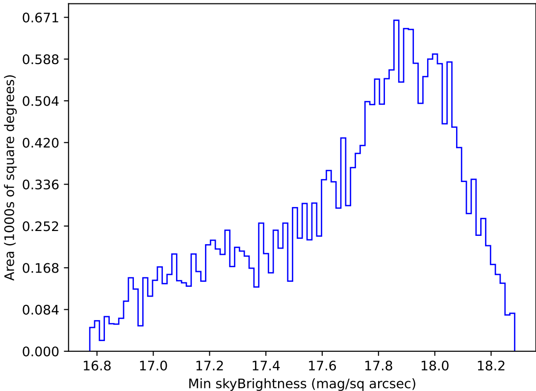
roll_pause_mjdp60_v3.4_10yrs Yr 1 y band: Min skyBrightness
