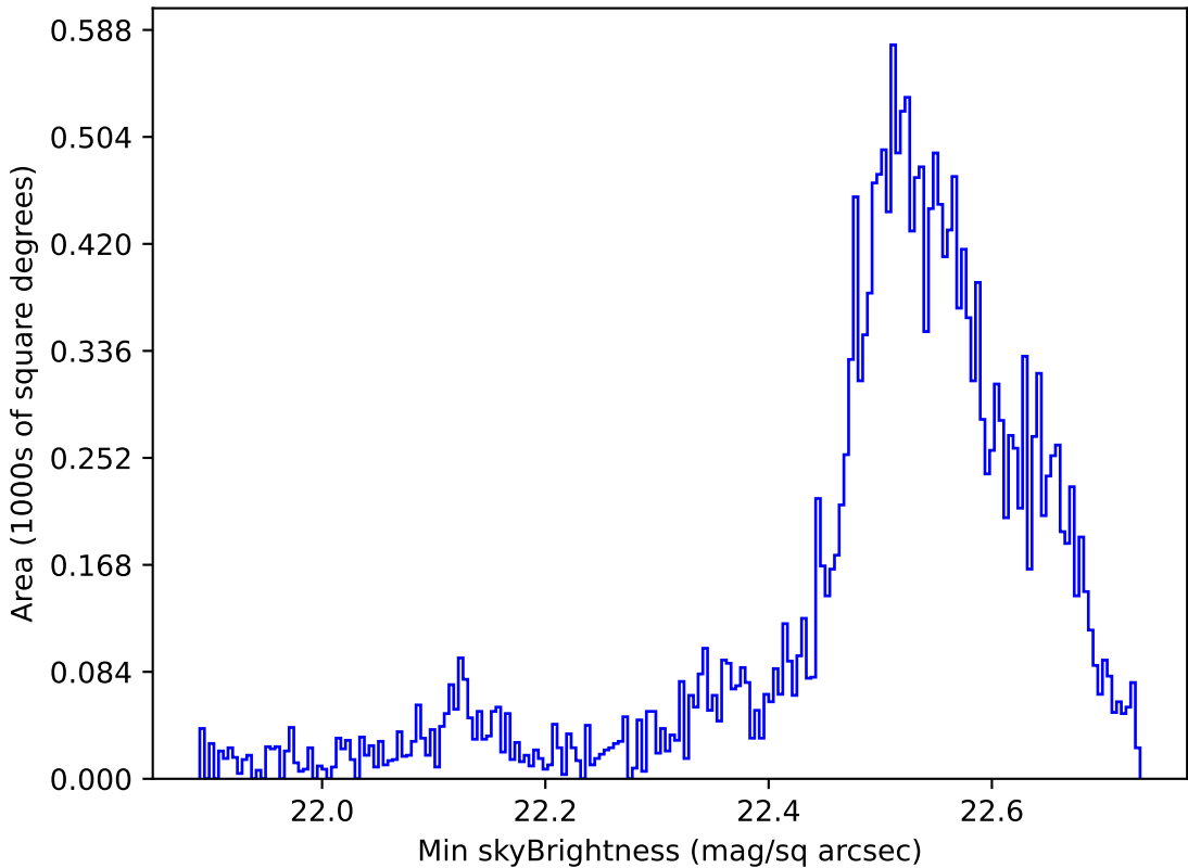
roll_pause_mjdp60_v3.4_10yrs Yr 1 u band: Min skyBrightness
