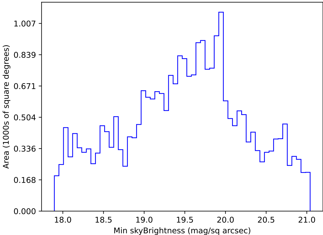
roll_pause_mjdp60_v3.4_10yrs Yr 1 r band: Min skyBrightness
