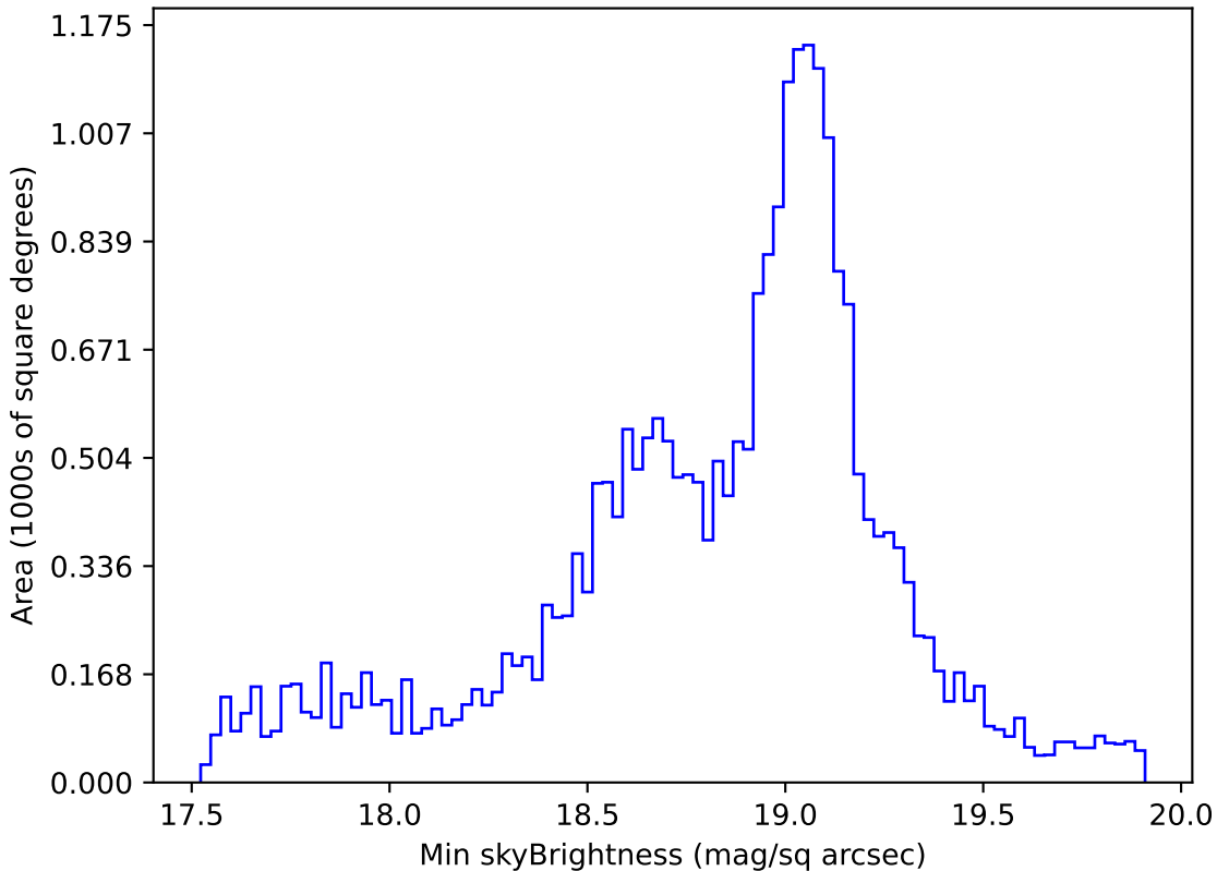
roll_pause_mjdp60_v3.4_10yrs Yr 1 i band: Min skyBrightness
