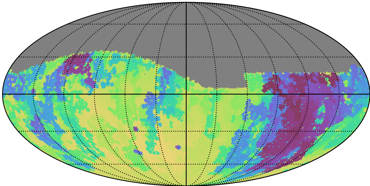
roll_pause_mjdp60_v3.4_10yrs Yr 1 g band: Min skyBrightness
