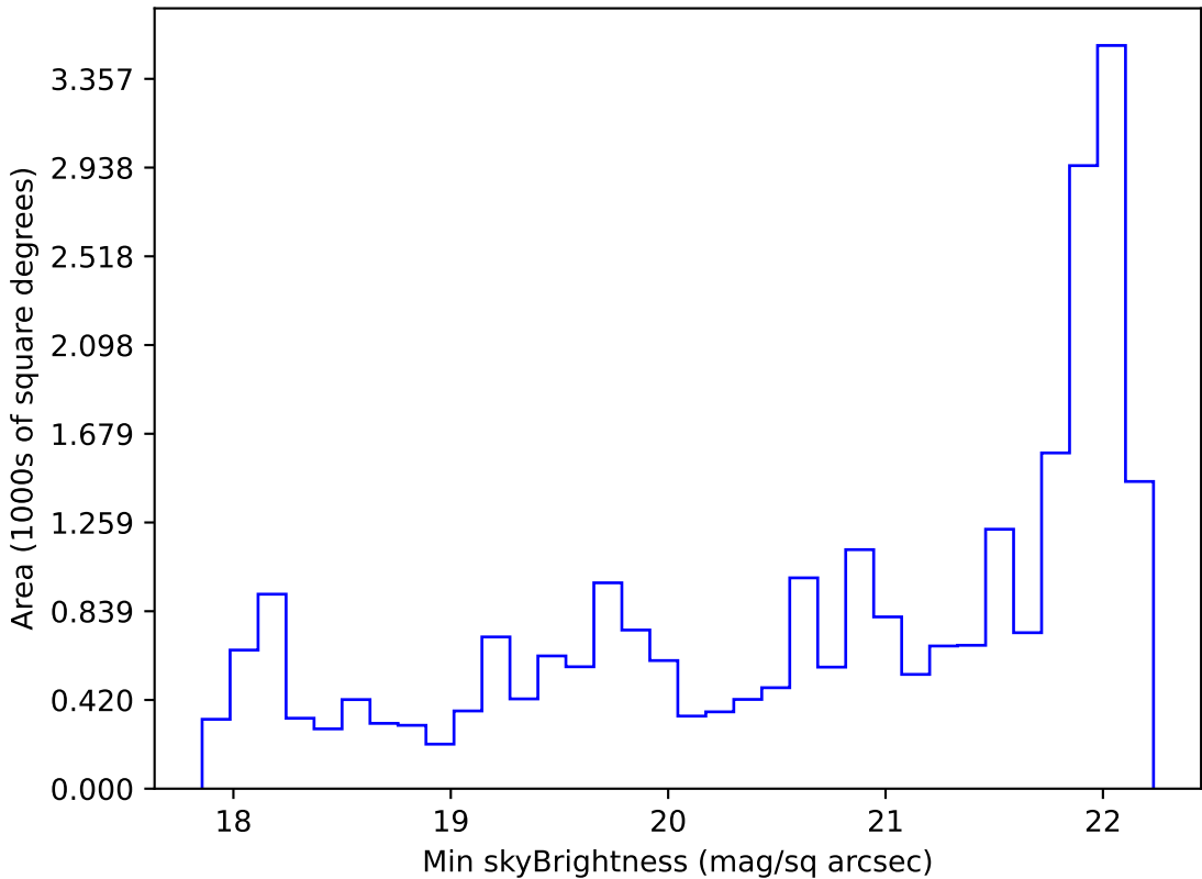
roll_pause_mjdp60_v3.4_10yrs Yr 1 g band: Min skyBrightness
