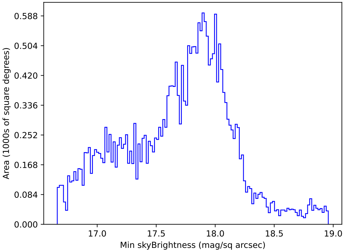
roll_pause_mjdp60_v3.4_10yrs Yr 1 all bands: Min skyBrightness
