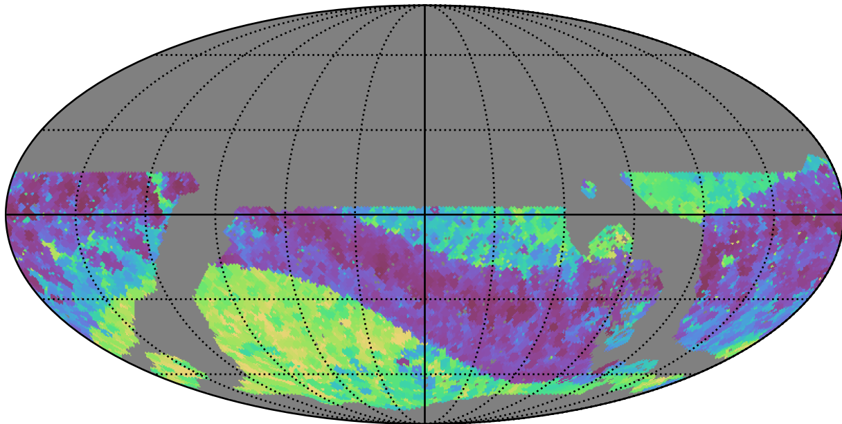
roll_pause_mjdp60_v3.4_10yrs WFD z band: Min skyBrightness
